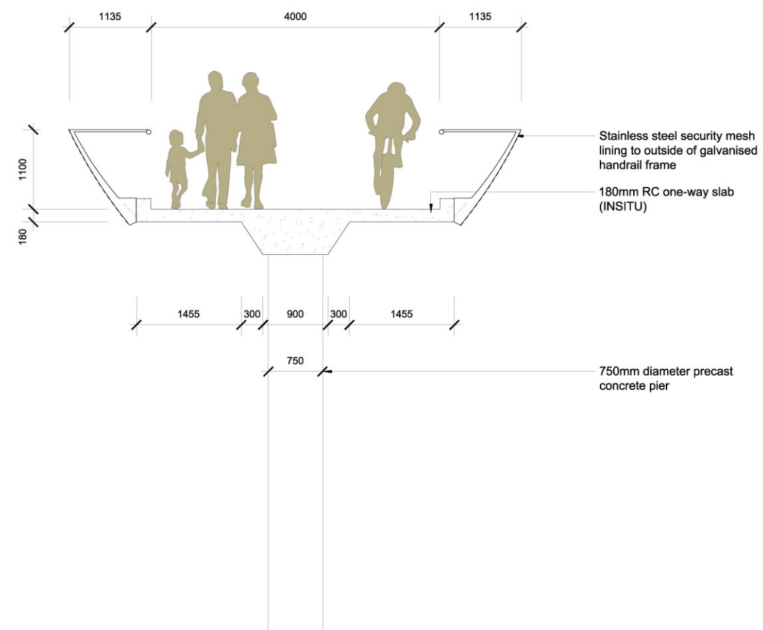
TYPICAL SECTION - RAMP
