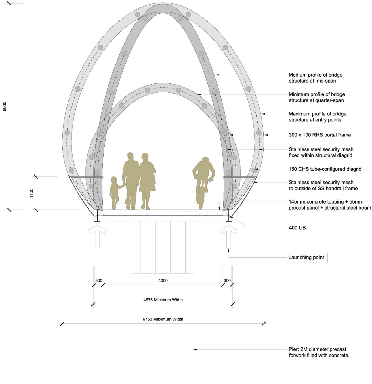
TYPICAL SECTION - BRIDGE
